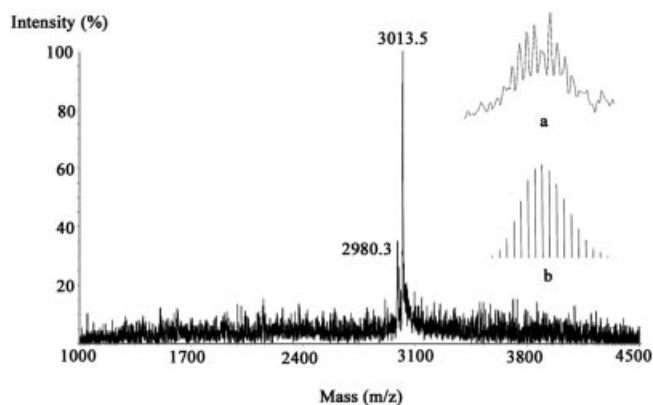
Figure 2. MALDI-TOF spectrum of 5 showing the major intensity peak at m/z = 3013.5 corresponding to [ 5 + H] + ; experimental (a) and simulated (b) isotope-distribution patterns are included; the peak at m/z = 2980 corresponds to [ 5 – S] +
