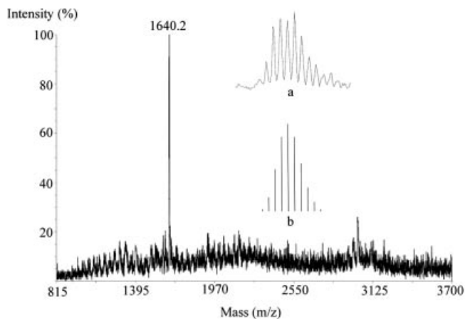
Figure 3. MALDI-TOF spectrum of 6 showing the major intensity peak at m/z = 1640.3 corresponding to [ 6 + 2 H] 2+ ; experimental (a) and simulated (b) isotope-distribution patterns are included
