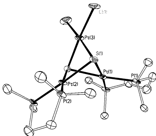
Figure 1. Molecular structure of 2 with the key atoms labeled and 50% probability ellipsoids; H atoms, phenyl rings and CH 2 Cl 2 solvent molecules have been omitted; selected structural parameters [Å, °]: Pt–Cl 2.330(7), Pt(1)–S 2.381(7), Pt(2)–S 2.357(6), Pt(3)–S 2.287(6), Pt(1)–P(1) 2.237(7), Pt(2)–P(2) 2.256(7), Pt(1)–Pt(2) 3.124(2), Pt(1)–Pt(3) 2.942(2), Pt(2)–Pt(3) 3.277(2), S–S 2.981; Cl–Pt(3)–Cl 91.1(4), P–Pt(1)–P 93.6(4), P–Pt(2)–P 93.1(3), S–Pt(1)–S 77.5(3), S–Pt(2)–S 78.5(3), S–Pt(3)–S 81.4(3); dihedral (hinge) angles between PtS 2 planes: Pt(1)/Pt(2) 116.0, Pt(1)/Pt(3) 110.1, Pt(2)/Pt(3) 134.0
